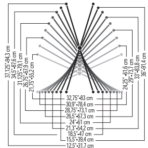
T/10 - T/10KD - T/20 Height & width positions
